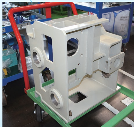
Drive unit frame
